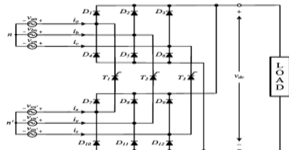
Figure.4. Proposed rectifier circuit.
