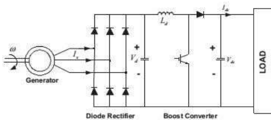
Figure.3. Diode bridge rectifier with dc-dc boost converter.
