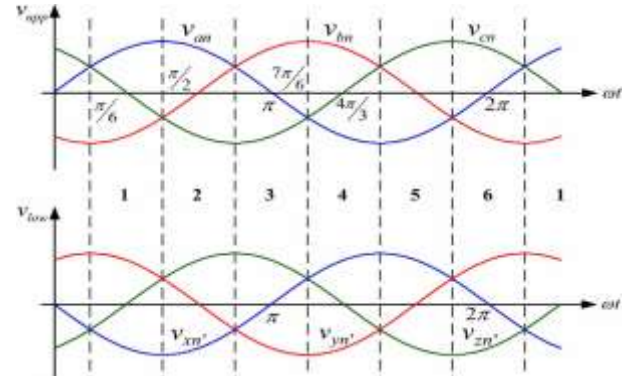
Figure.5. Input voltage supplied to the proposed rectifier.
