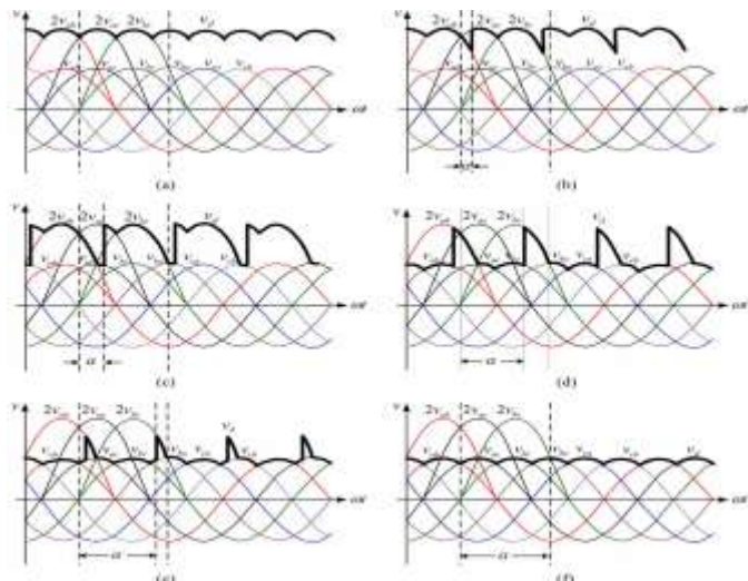
Fig. 6. Typical rectifier output waveforms. (a) \alpha = 0^\circ . (b) 0^\circ < \alpha < 30^\circ . (c) 30^\circ < \alpha < 60^\circ . (d) 60^\circ < \alpha < 120^\circ . (e) 120^\circ < \alpha < 150^\circ . (f) \alpha = 150^\circ .
