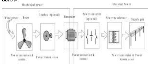
Figure.1. Main components of a wind turbine
