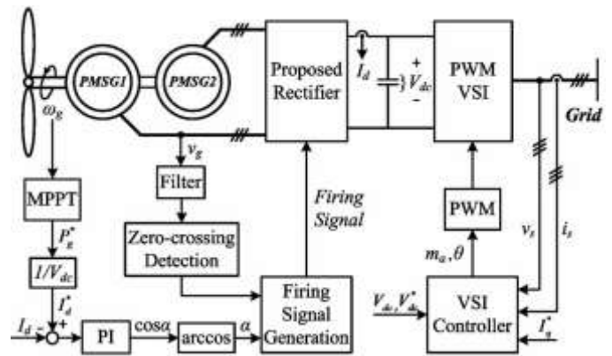
Fig. 7. MPPT control of PMSG wind turbine with the proposed rectifier.
