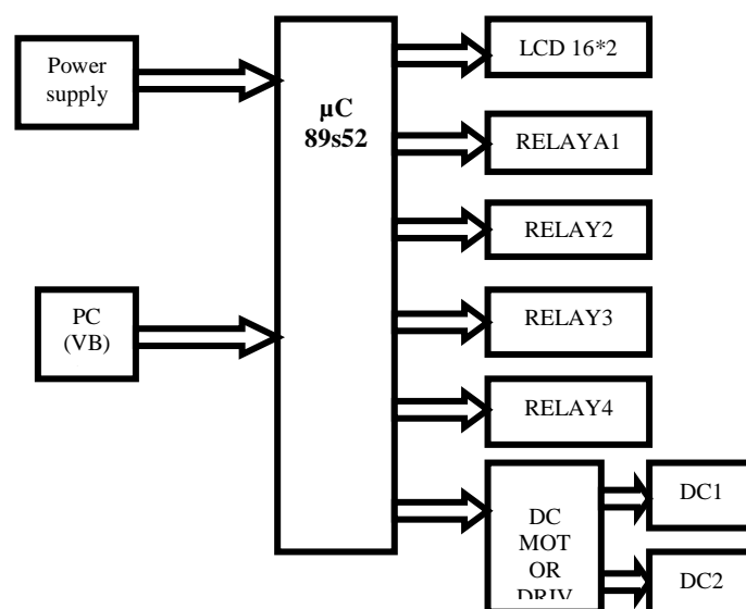
Figure 1: Basic Block Diagram
