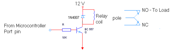
Figure 5: Internal relay driver circuit.[6]
