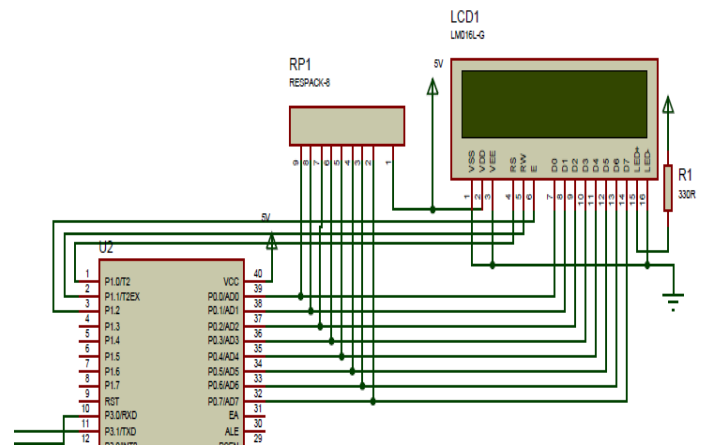
Figure3: LCD interfacing with micrcontroller
