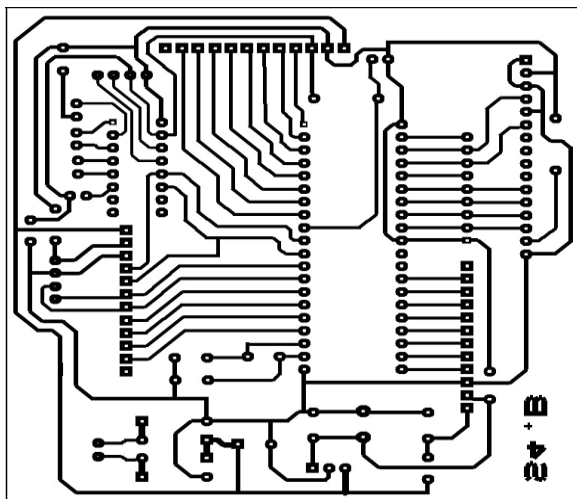
Figure 11: PCB layout of circuit
