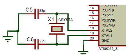
Figure 8: Connection of Crystal Circuit
